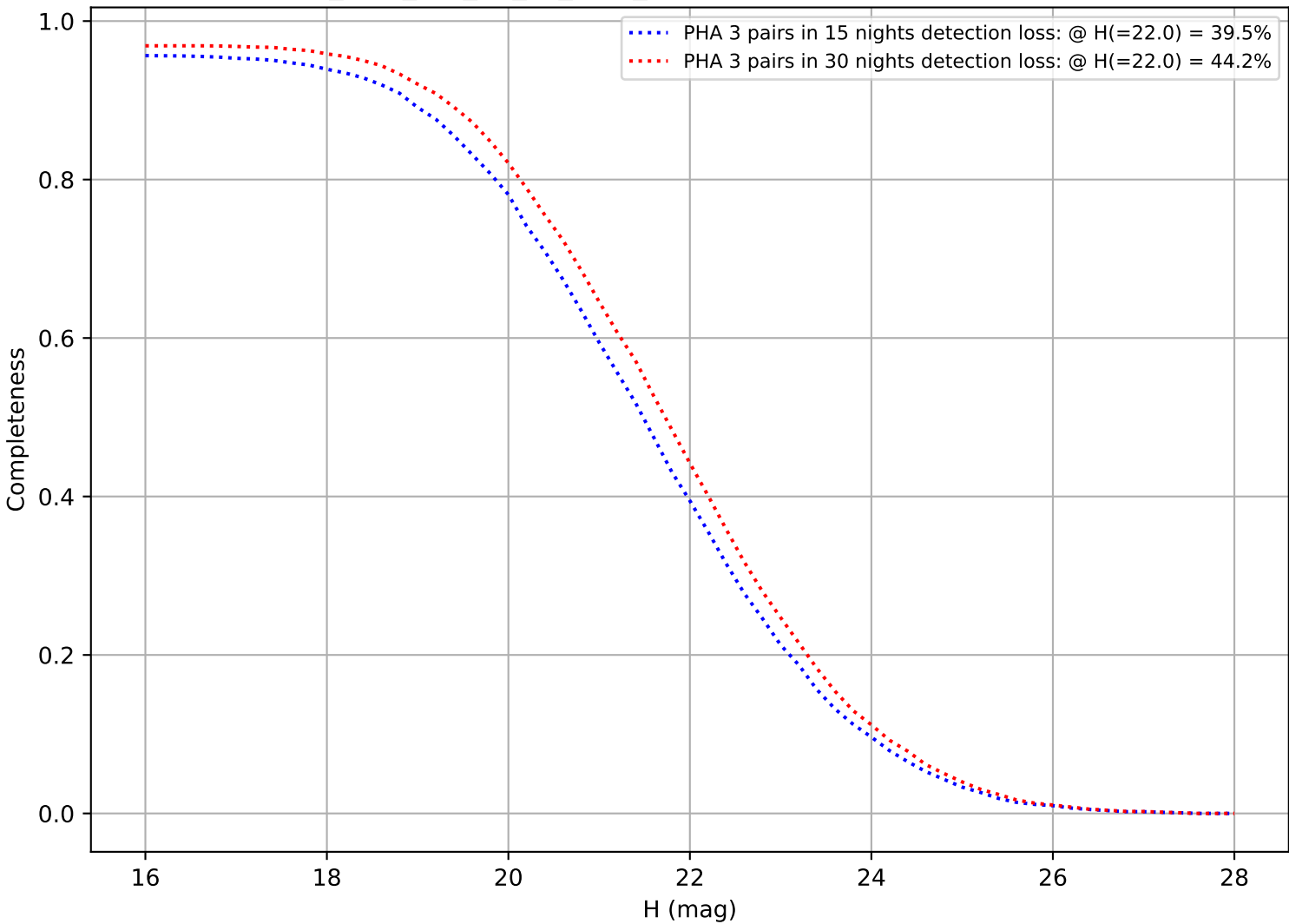
too_elab_r16_d3_gz_v3.4_10yrs: DifferentialCompleteness
