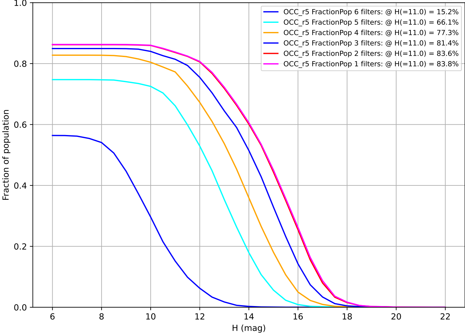
too_elab_r16_d3_gz_v3.4_10yrs: Fraction of population with colors in X filters OCC_r5
