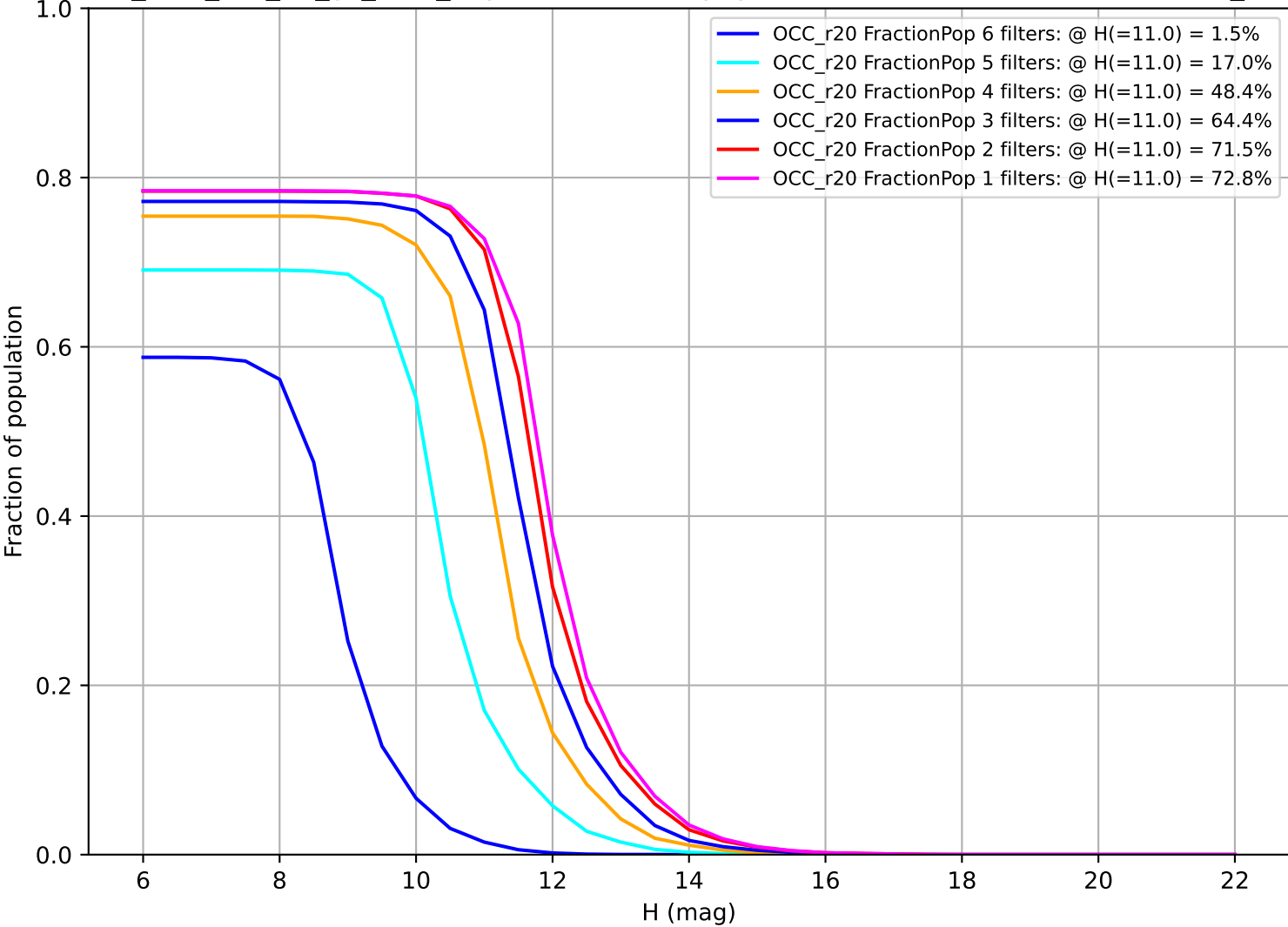
too_elab_r16_d3_gz_v3.4_10yrs: Fraction of population with colors in X filters OCC_r20
