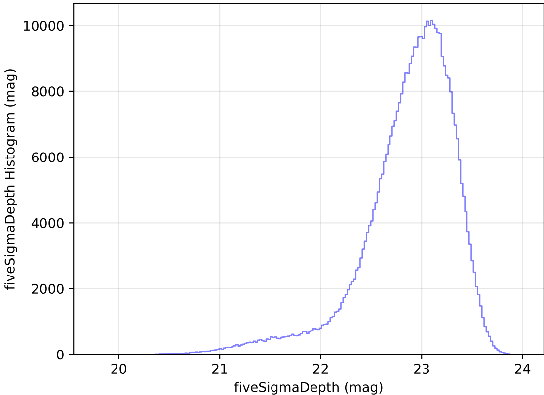
too_elab_r16_d3_gz_v3.4_10yrs z: fiveSigmaDepth Histogram
