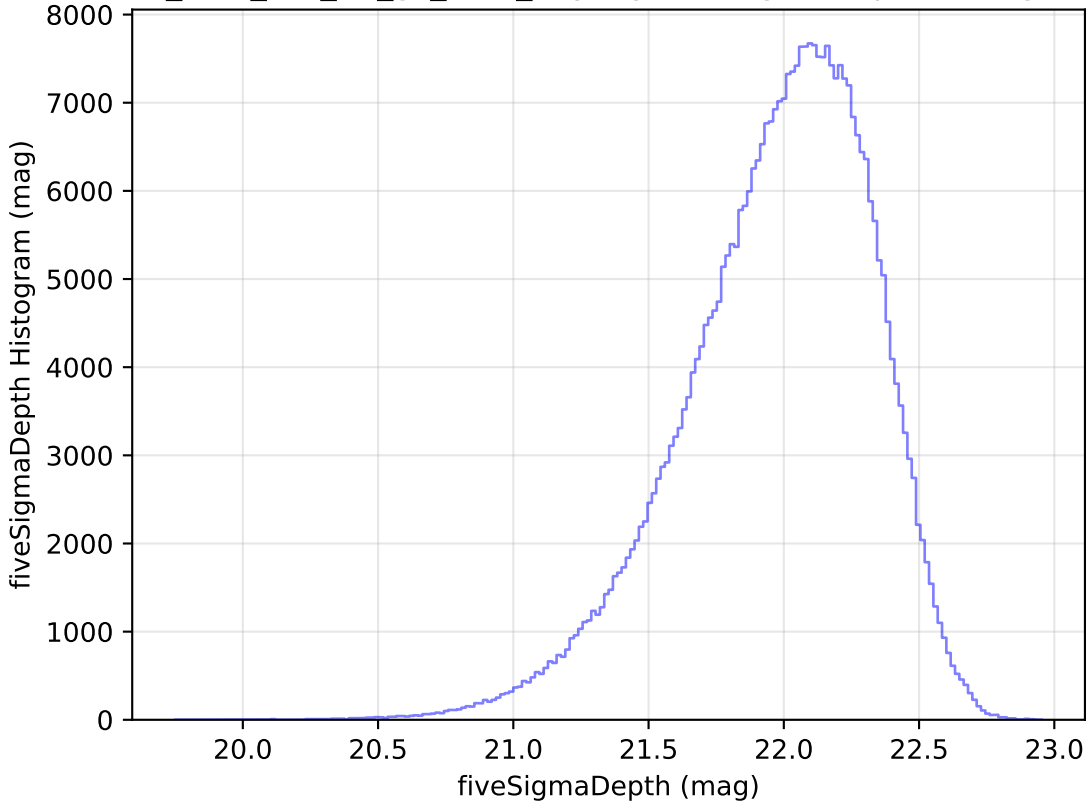
too_elab_r16_d3_gz_v3.4_10yrs y: fiveSigmaDepth Histogram
