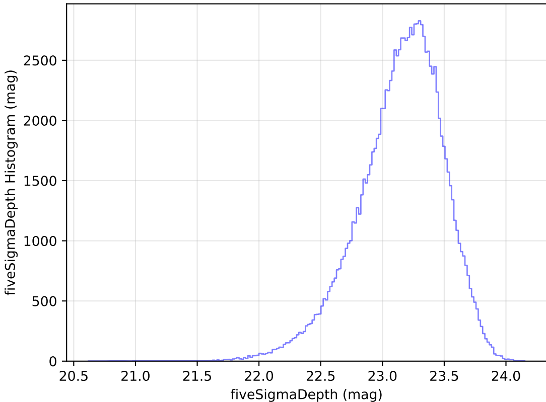
too_elab_r16_d3_gz_v3.4_10yrs u: fiveSigmaDepth Histogram
