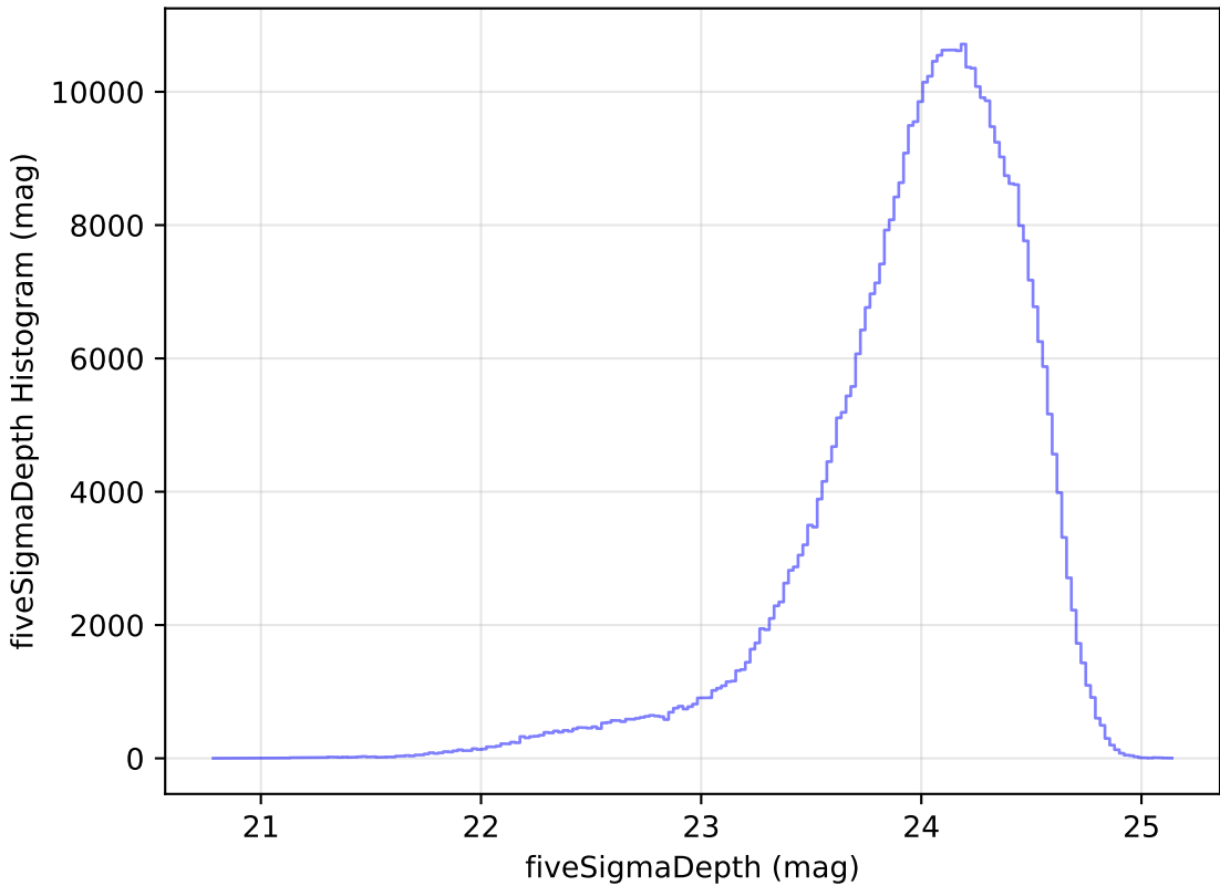
too_elab_r16_d3_gz_v3.4_10yrs r: fiveSigmaDepth Histogram
