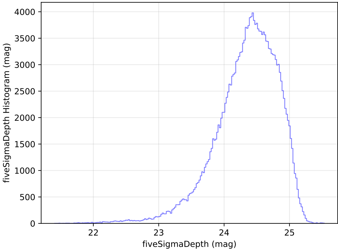
too_elab_r16_d3_gz_v3.4_10yrs g: fiveSigmaDepth Histogram
