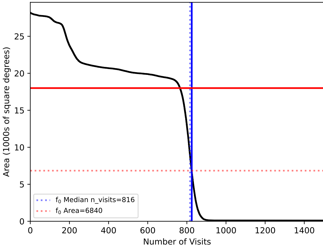
too_elab_r16_d3_gz_v3.4_10yrs : f0
