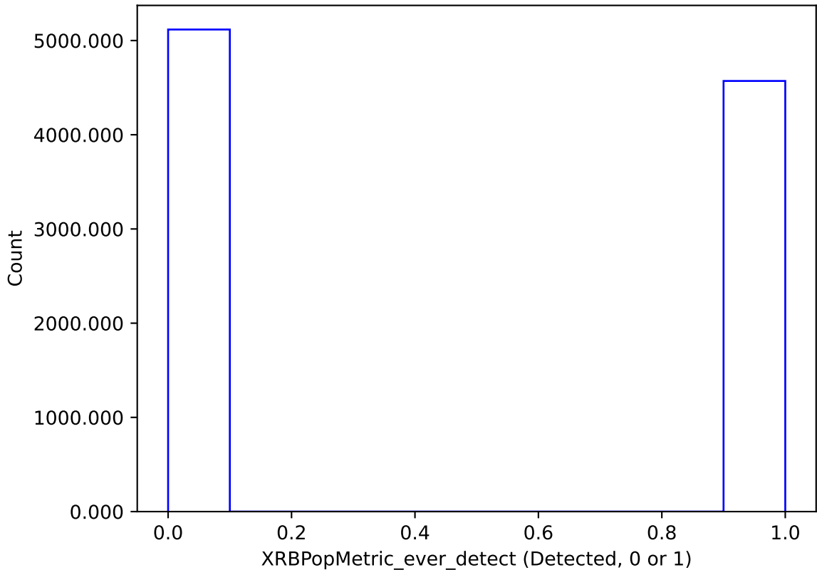
too_elab_r16_d3_gz_v3.4_10yrs : XRBPoMetric_ever_detect
