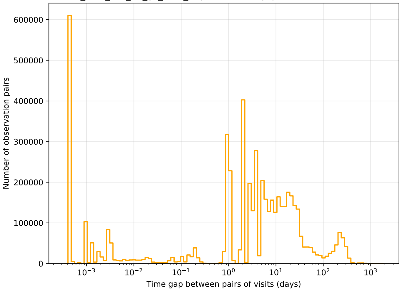
too_elab_r16_d3_gz_v3.4_10yrs r band: Tgaps observationStartMJD
