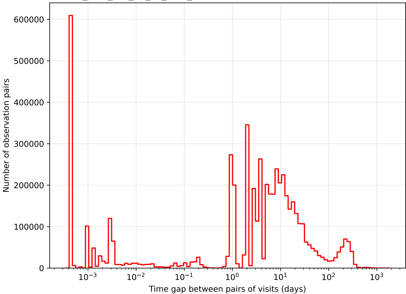
too_elab_r16_d3_gz_v3.4_10yrs i band: Tgaps observationStartMJD
