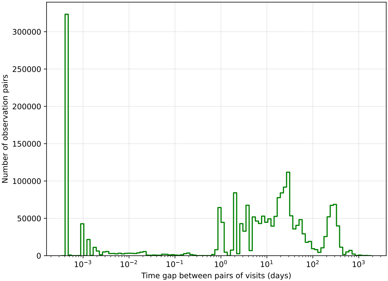
too_elab_r16_d3_gz_v3.4_10yrs g band: Tgaps observationStartMJD
