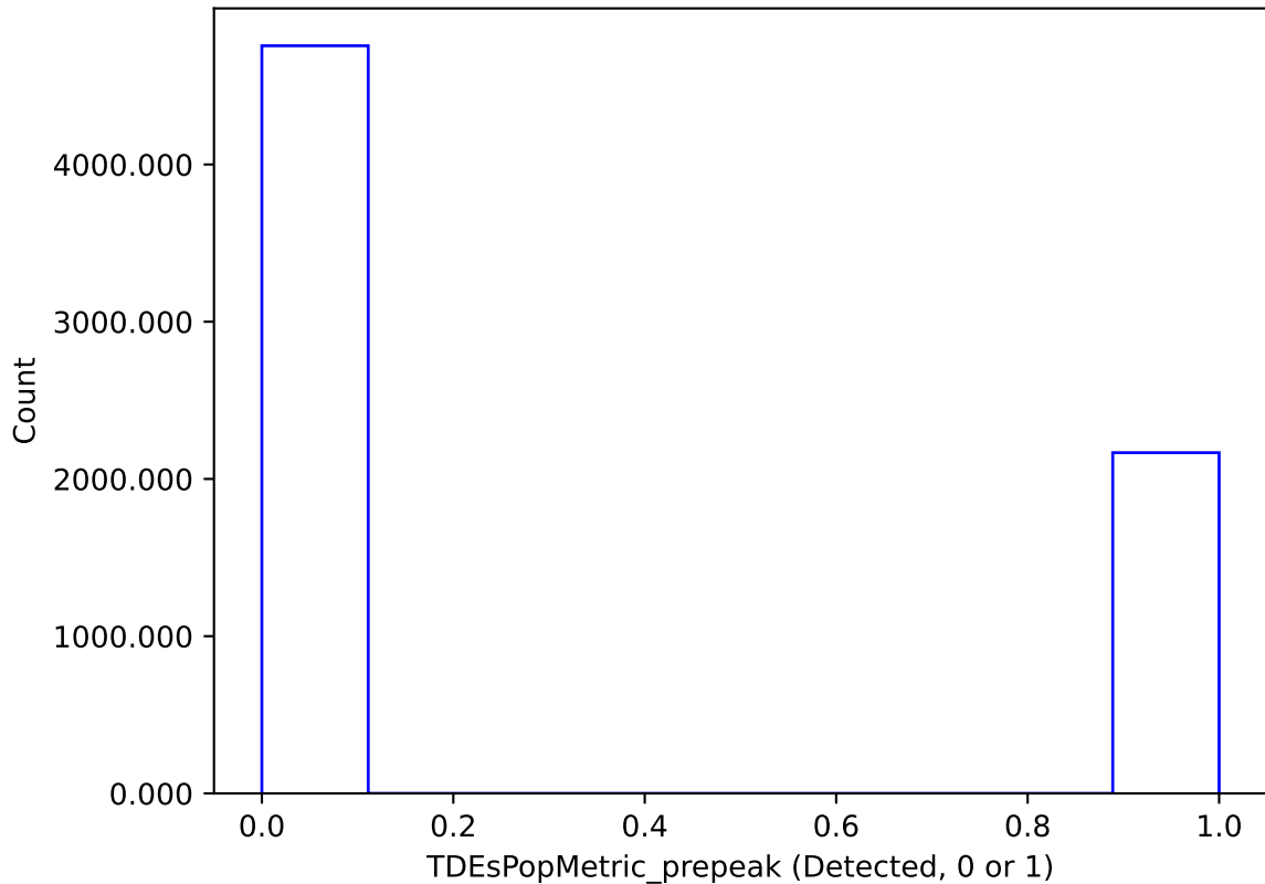
too_elab_r16_d3_gz_v3.4_10yrs : TDEsPopMetric_prepeak
