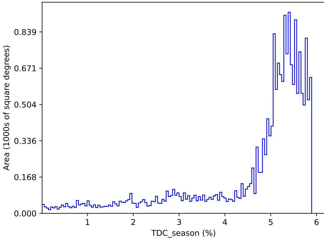
too_elab_r16_d3_gz_v3.4_10yrs : TDC_season
