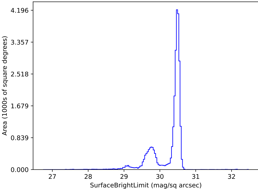
too_elab_r16_d3_gz_v3.4_10yrs r: SurfaceBrightLimit
