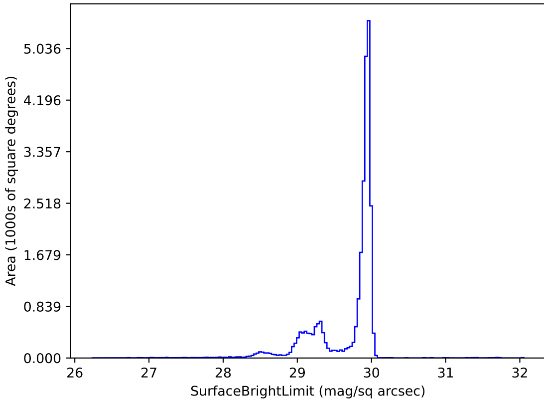
too_elab_r16_d3_gz_v3.4_10yrs i: SurfaceBrightLimit
