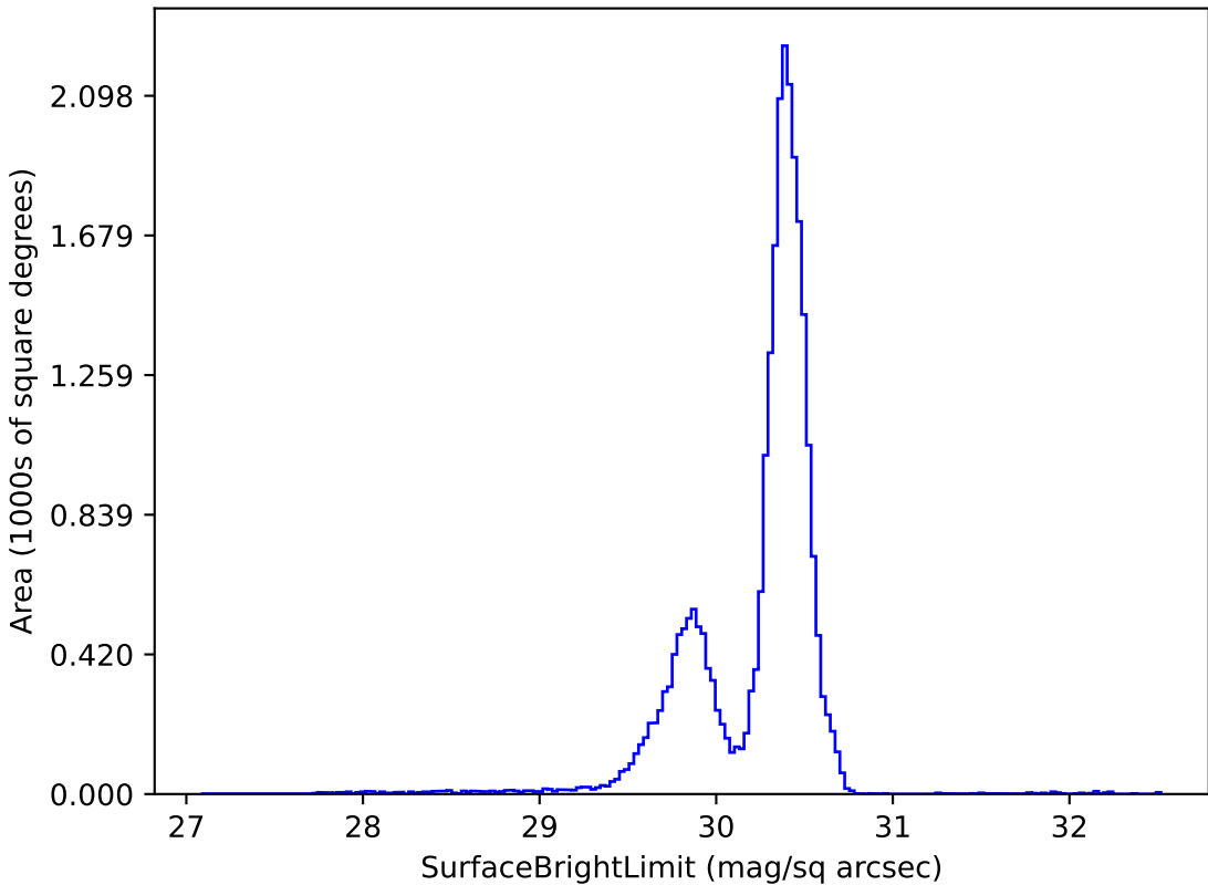
too_elab_r16_d3_gz_v3.4_10yrs g: SurfaceBrightLimit
