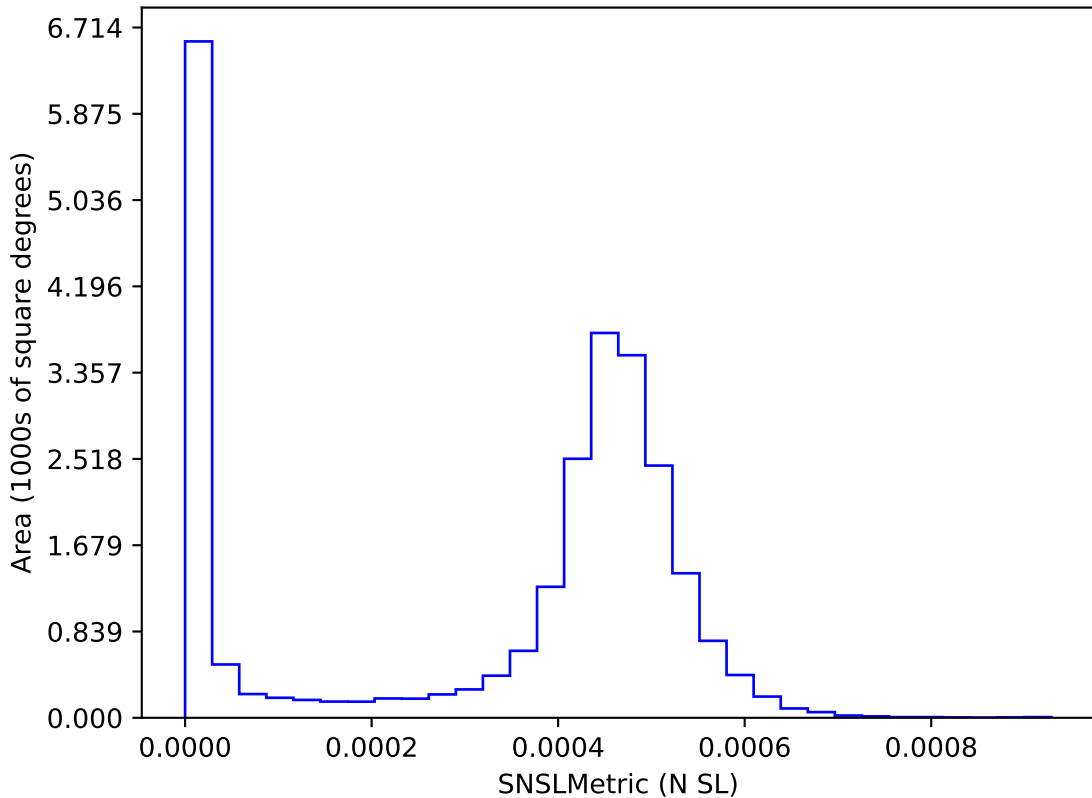
too_elab_r16_d3_gz_v3.4_10yrs : SNSLMetric
