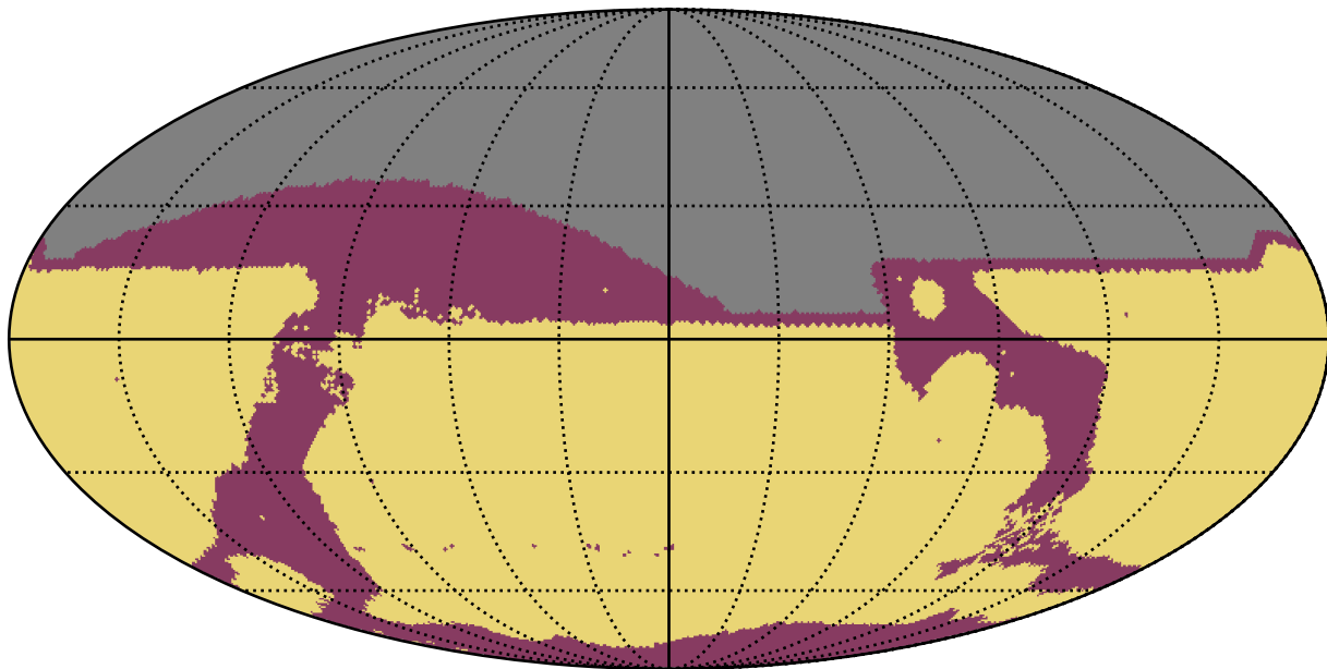
too_elab_r16_d3_gz_v3.4_10yrs : RapidRevisits
