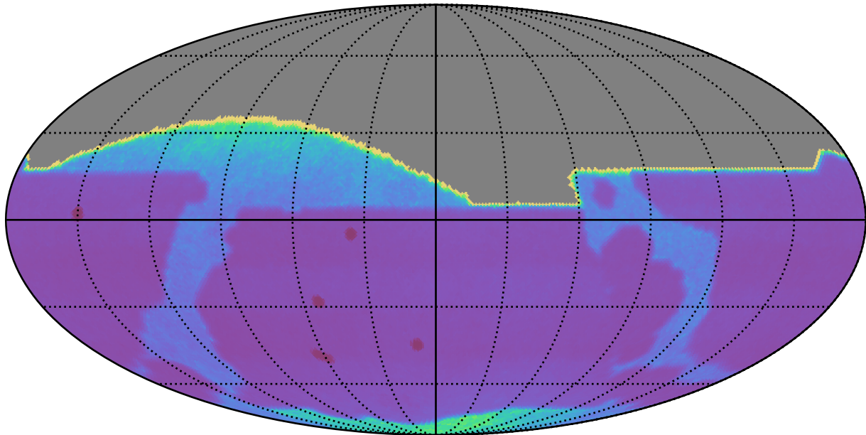
too_elab_r16_d3_gz_v3.4_10yrs : Proper Motion Uncert @ 20.5
