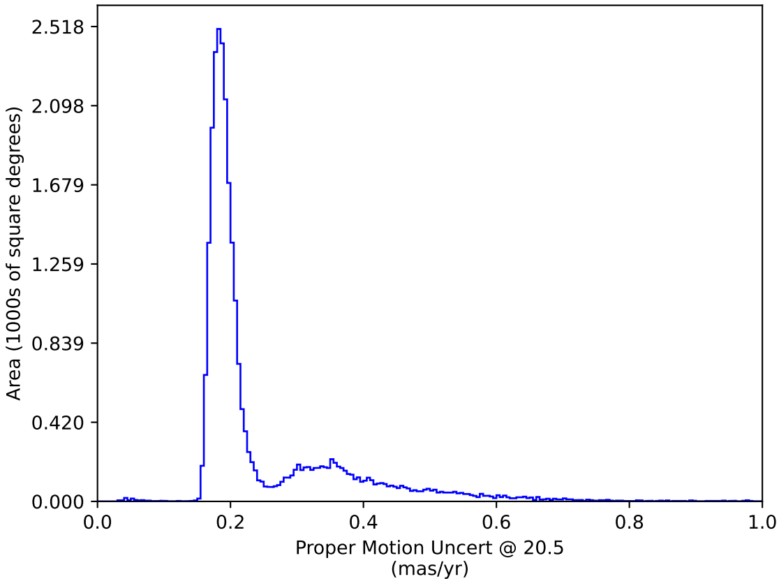
too_elab_r16_d3_gz_v3.4_10yrs : Proper Motion Uncert @ 20.5
