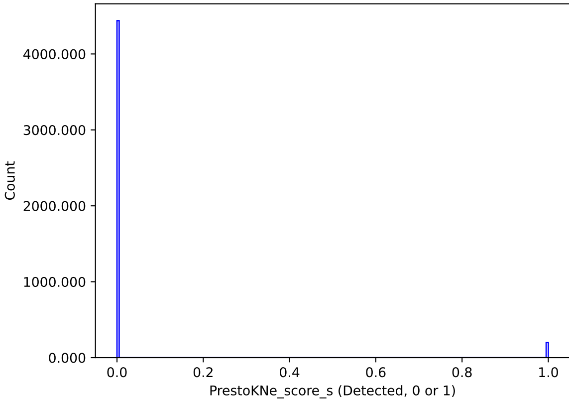
too_elab_r16_d3_gz_v3.4_10yrs : PrestoKNe_score_s
