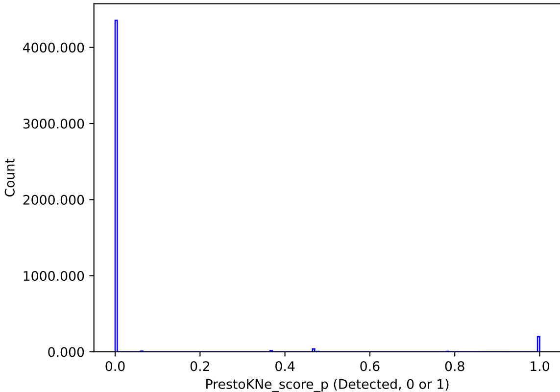
too_elab_r16_d3_gz_v3.4_10yrs : PrestoKNe_score_p
