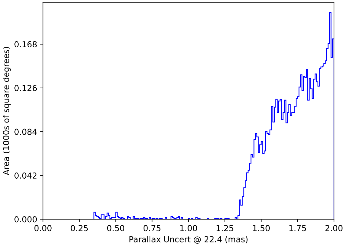
too_elab_r16_d3_gz_v3.4_10yrs : Parallax Uncert @ 22.4
