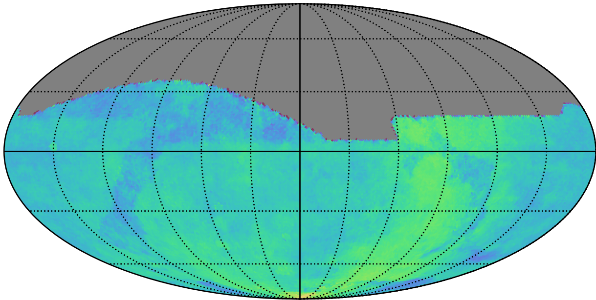
too_elab_r16_d3_gz_v3.4_10yrs : Parallax Coverage @ 24.0
