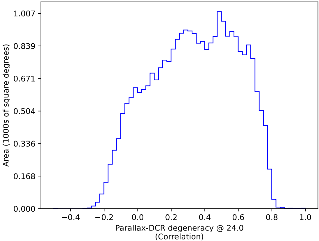
too_elab_r16_d3_gz_v3.4_10yrs : Parallax-DCR degeneracy @ 24.0
