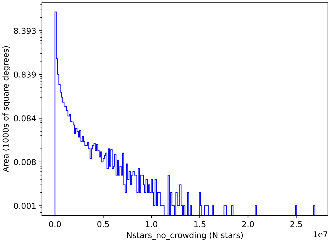
too_elab_r16_d3_gz_v3.4_10yrs i: Nstars_no_crowding
