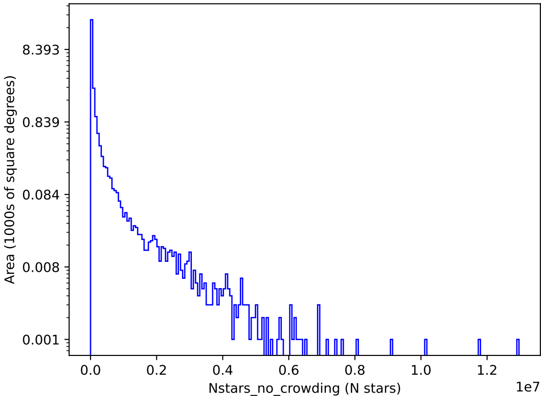
too_elab_r16_d3_gz_v3.4_10yrs g: Nstars_no_crowding
