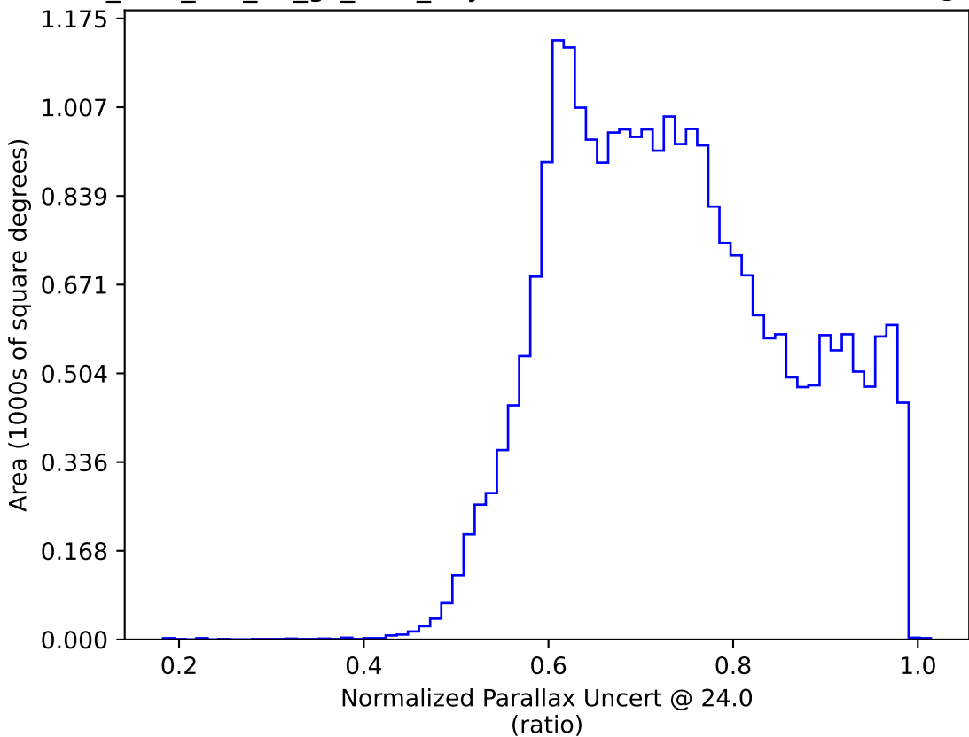
too_elab_r16_d3_gz_v3.4_10yrs : Normalized Parallax Uncert @ 24.0
