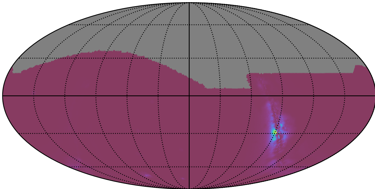
too_elab_r16_d3_gz_v3.4_10yrs : NlcPoints
