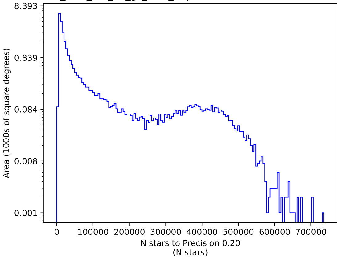
too_elab_r16_d3_gz_v3.4_10yrs z: N stars to Precision 0.20
