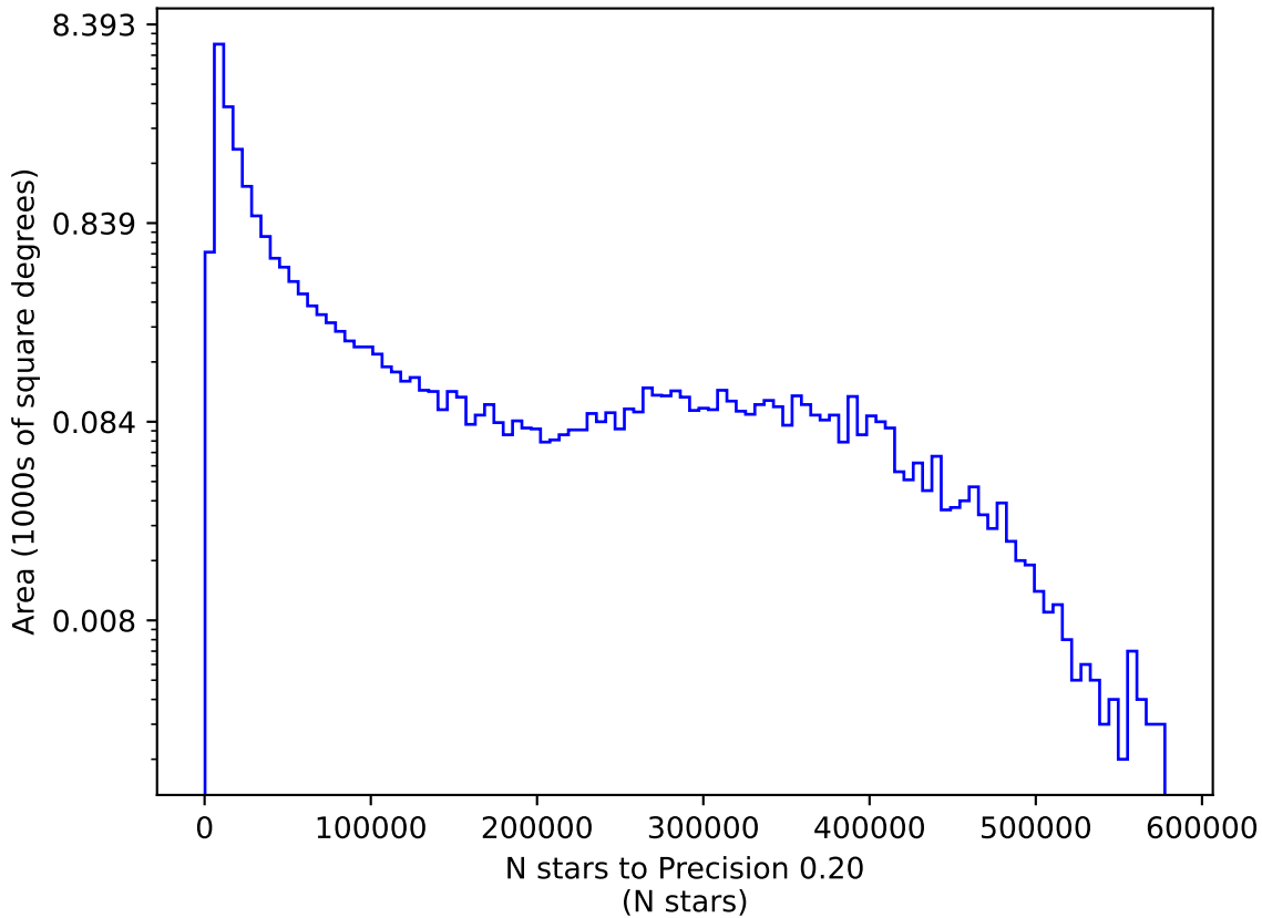
too_elab_r16_d3_gz_v3.4_10yrs y: N stars to Precision 0.20
