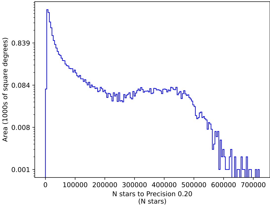
too_elab_r16_d3_gz_v3.4_10yrs r: N stars to Precision 0.20
