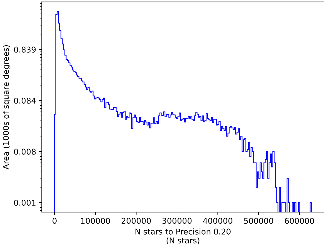
too_elab_r16_d3_gz_v3.4_10yrs g: N stars to Precision 0.20
