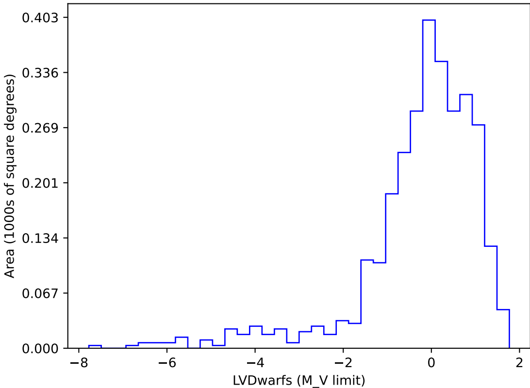
too_elab_r16_d3_gz_v3.4_10yrs gi SCP: LVDwarfs
