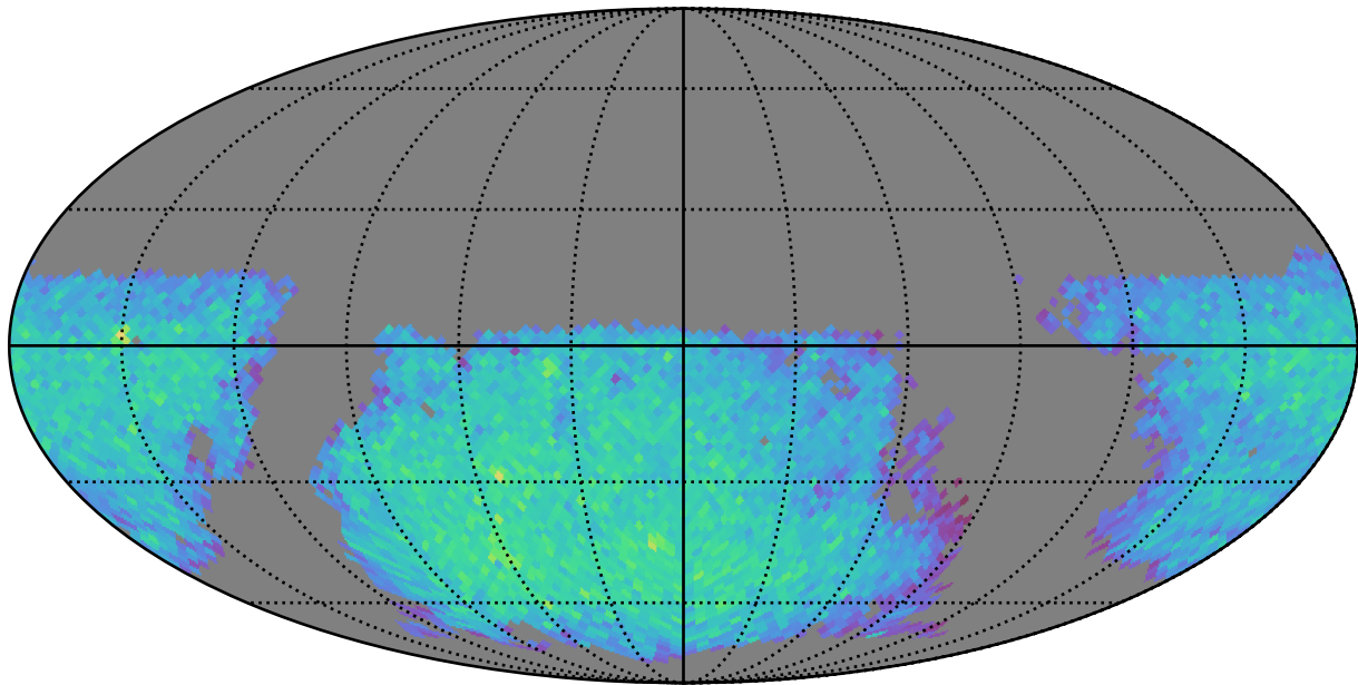
too_elab_r16_d3_gz_v3.4_10yrs gi: LVDwarfs
