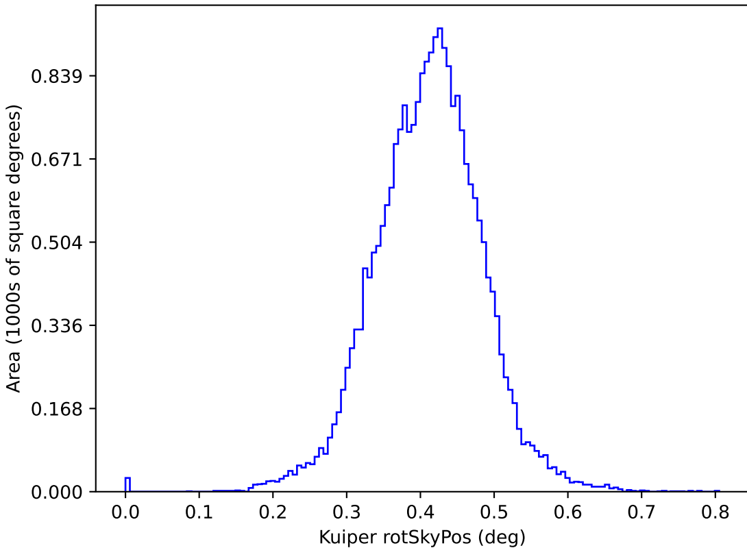
too_elab_r16_d3_gz_v3.4_10yrs y: Kuiper rotSkyPos
