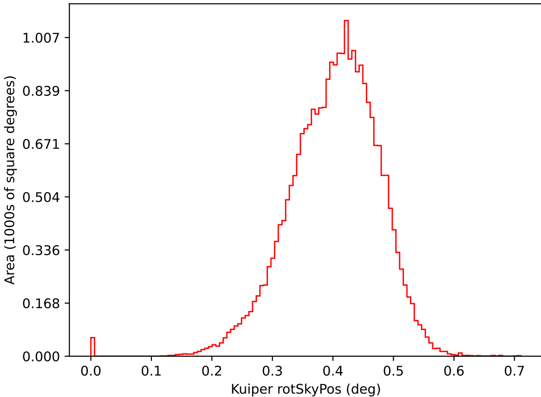
too_elab_r16_d3_gz_v3.4_10yrs i: Kuiper rotSkyPos
