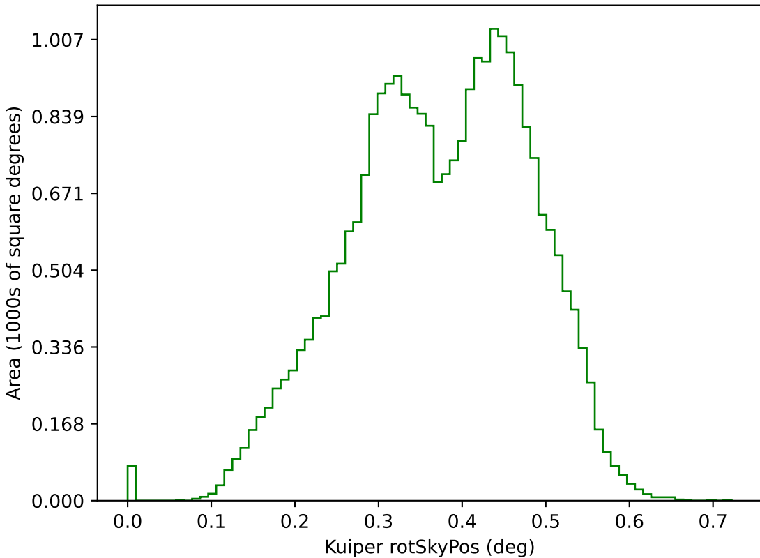
too_elab_r16_d3_gz_v3.4_10yrs g: Kuiper rotSkyPos
