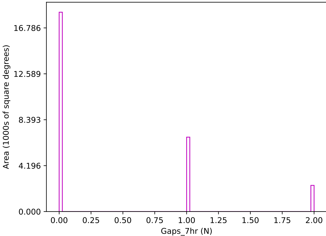
too_elab_r16_d3_gz_v3.4_10yrs z band: Gaps_7hr
