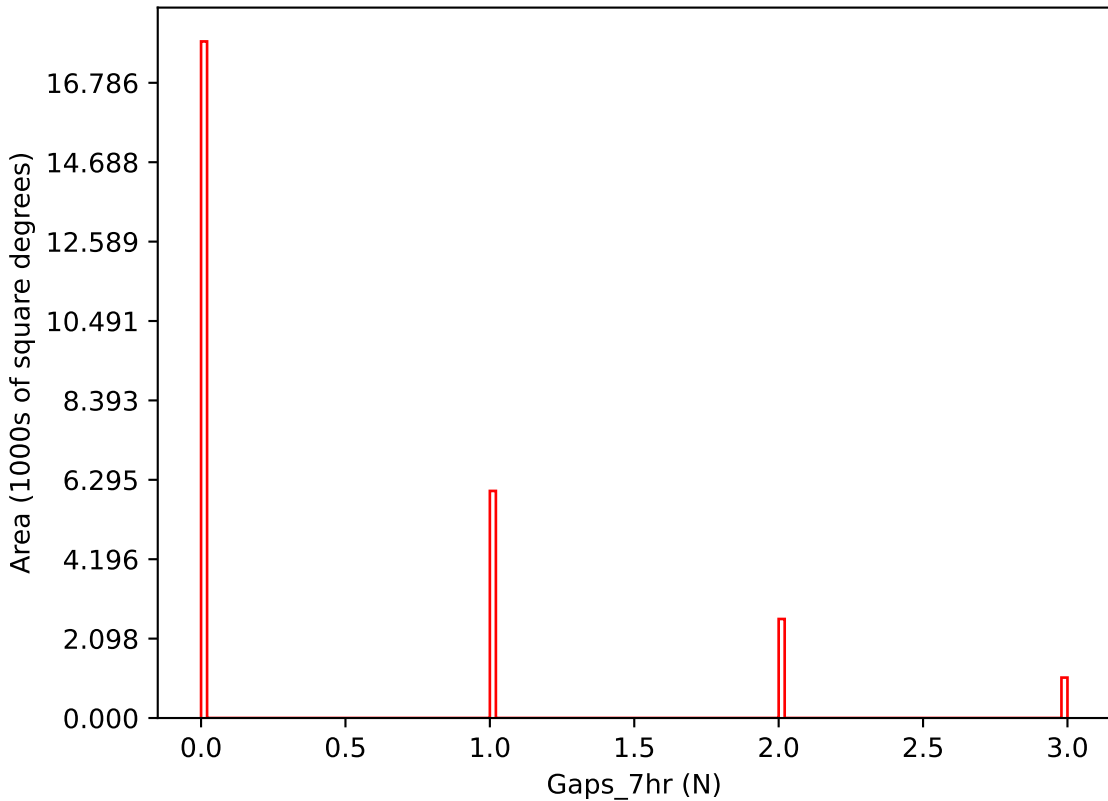
too_elab_r16_d3_gz_v3.4_10yrs i band: Gaps_7hr
