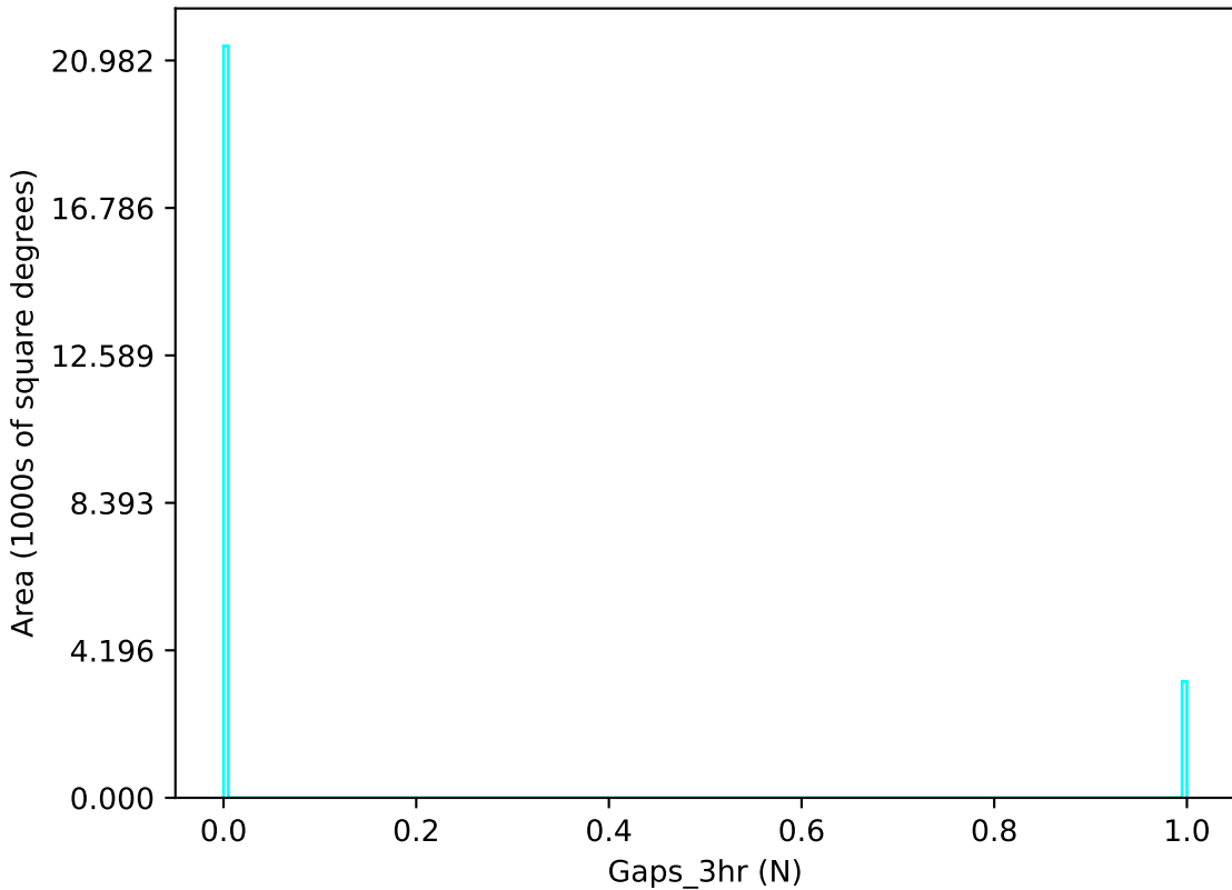
too_elab_r16_d3_gz_v3.4_10yrs u band: Gaps_3hr
