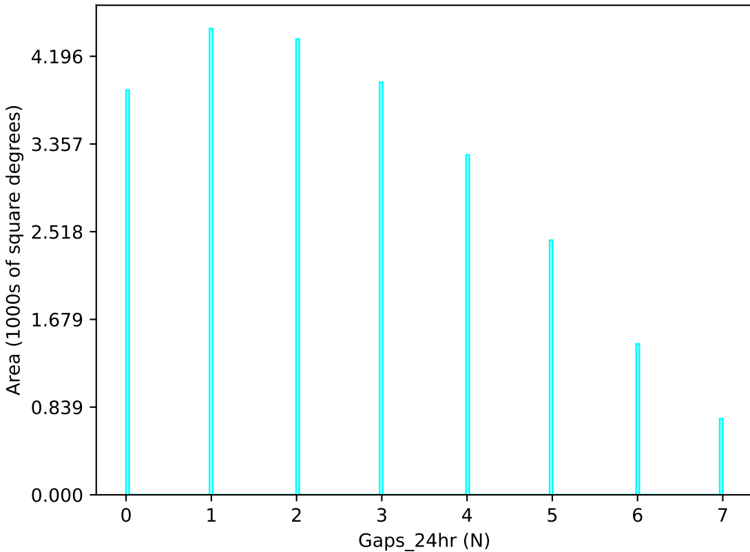
too_elab_r16_d3_gz_v3.4_10yrs u band: Gaps_24hr
