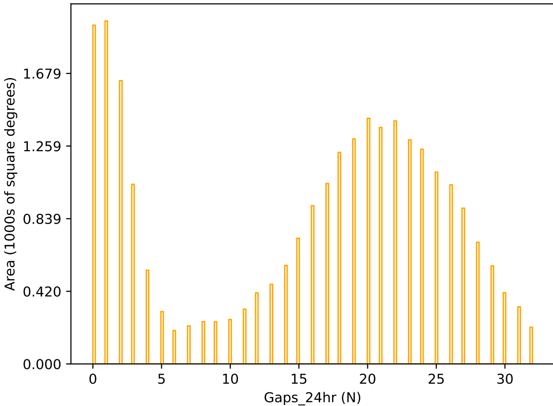
too_elab_r16_d3_gz_v3.4_10yrs r band: Gaps_24hr
