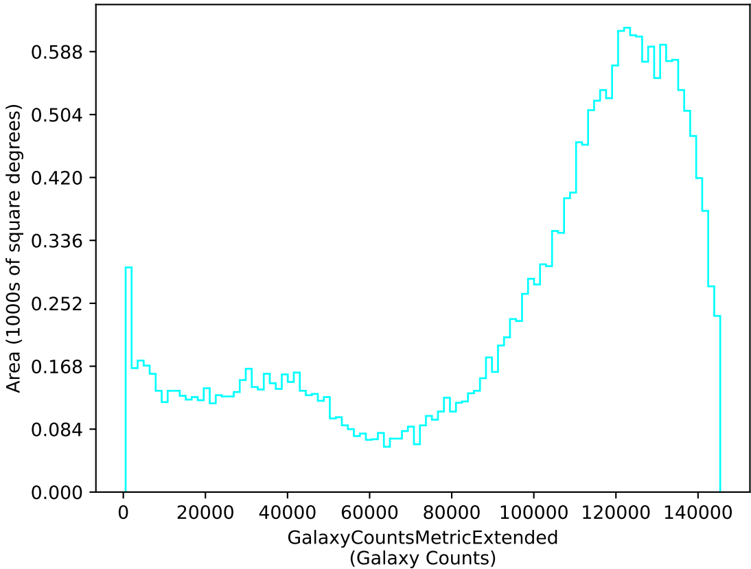
too_elab_r16_d3_gz_v3.4_10yrs u: GalaxyCountsMetricExtended
