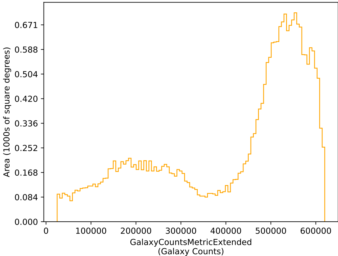
too_elab_r16_d3_gz_v3.4_10yrs r: GalaxyCountsMetricExtended
