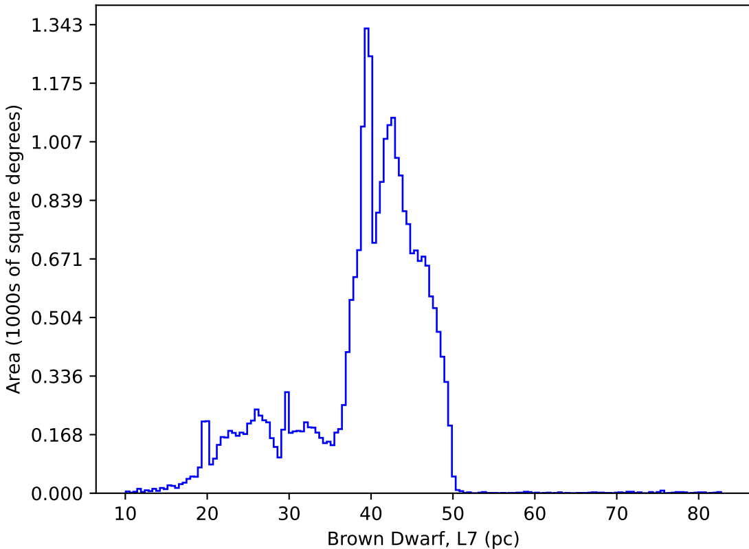
too_elab_r16_d3_gz_v3.4_10yrs : Brown Dwarf, L7
