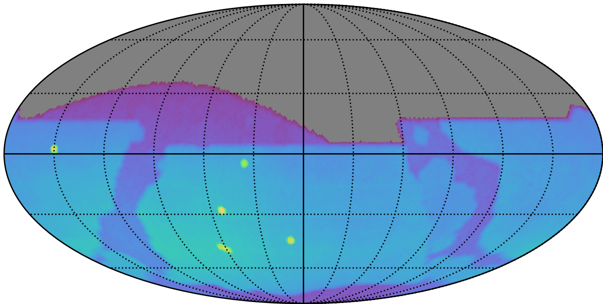
too_elab_r16_d3_gz_v3.4_10yrs : Brown Dwarf, L4
