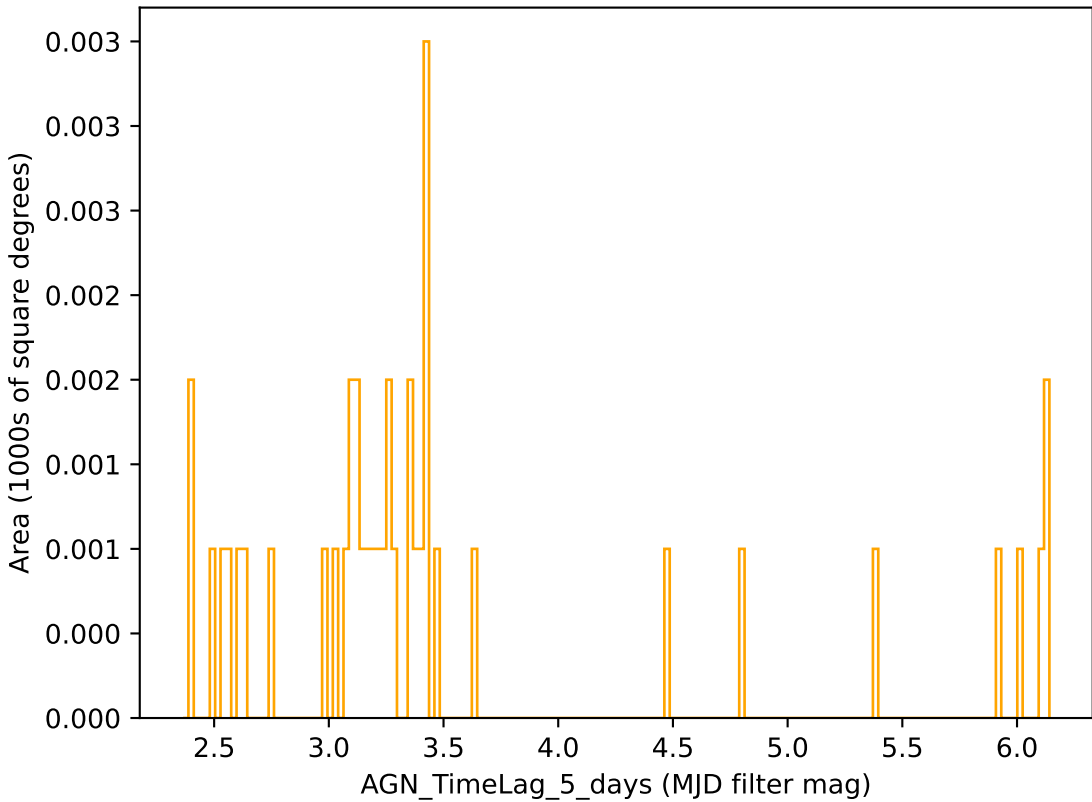
too_elab_r16_d3_gz_v3.4_10yrs r band: AGN_TimeLag_5_days
